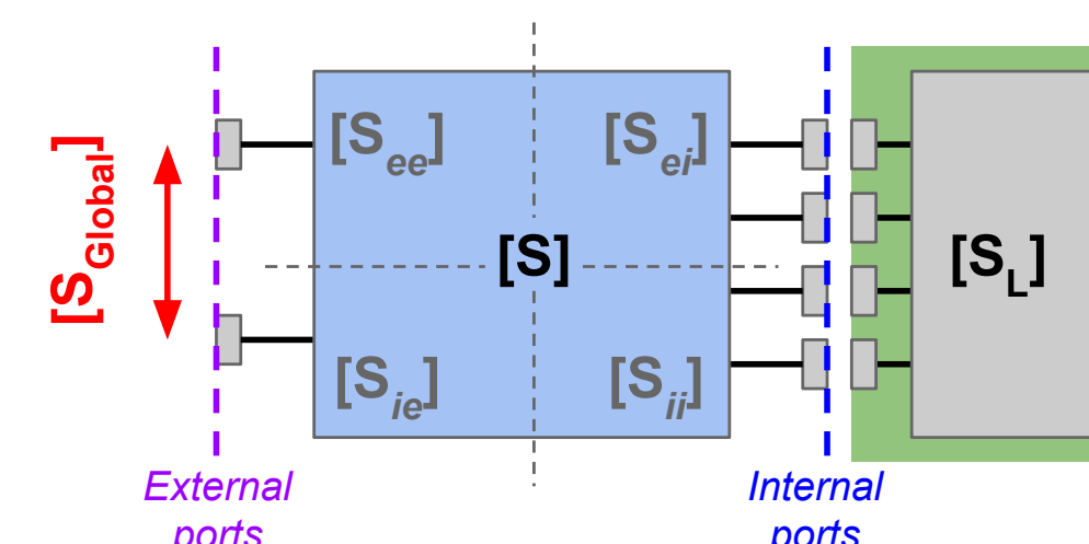
Figure 2: Illustration of an unbalanced multipoint S-parameters terminated with a multipoint load at its internal ports.
