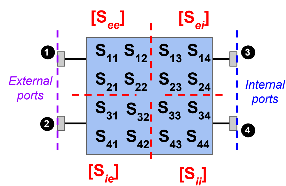
Figure 1: Example of partitioning on a balanced multipoint.
